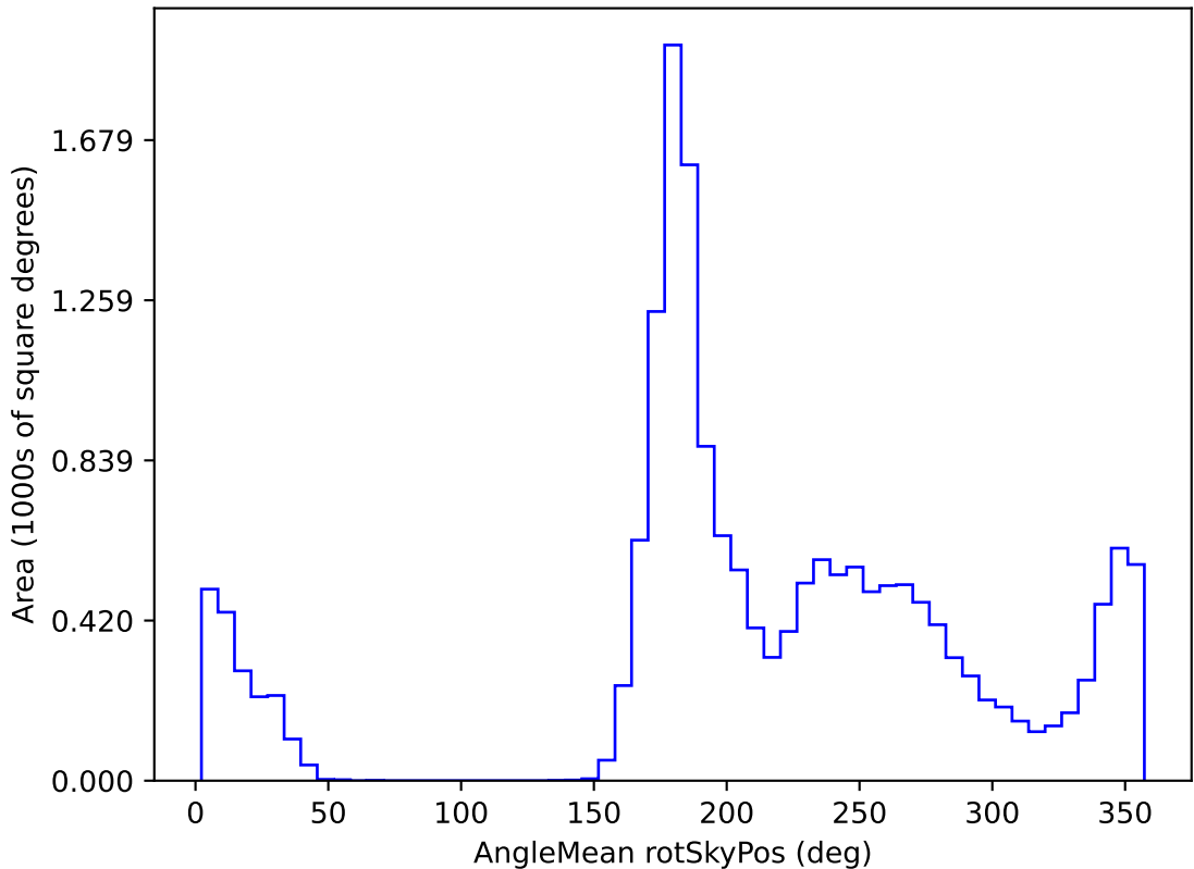
ddf_loaded_half_fl1_v3.4_10yrs WFD z band: AngleMean rotSkyPos
