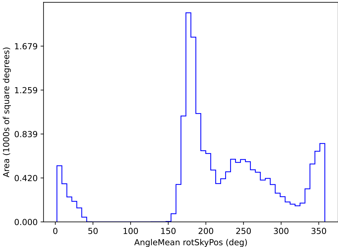
ddf_loaded_half_fl1_v3.4_10yrs WFD i band: AngleMean rotSkyPos
