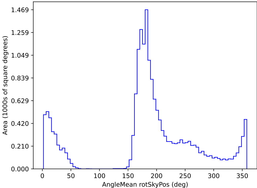
ddf_loaded_half_fl1_v3.4_10yrs WFD g band: AngleMean rotSkyPos
