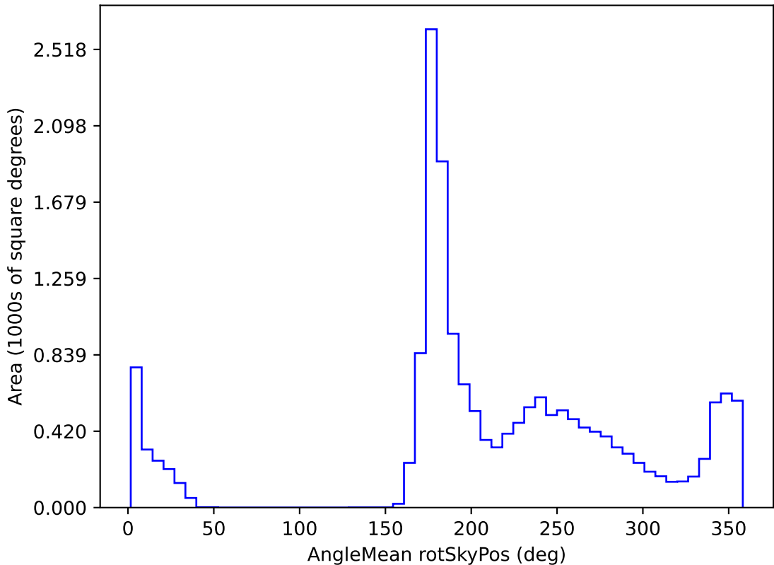
ddf_loaded_half_fl1_v3.4_10yrs WFD all bands: AngleMean rotSkyPos
