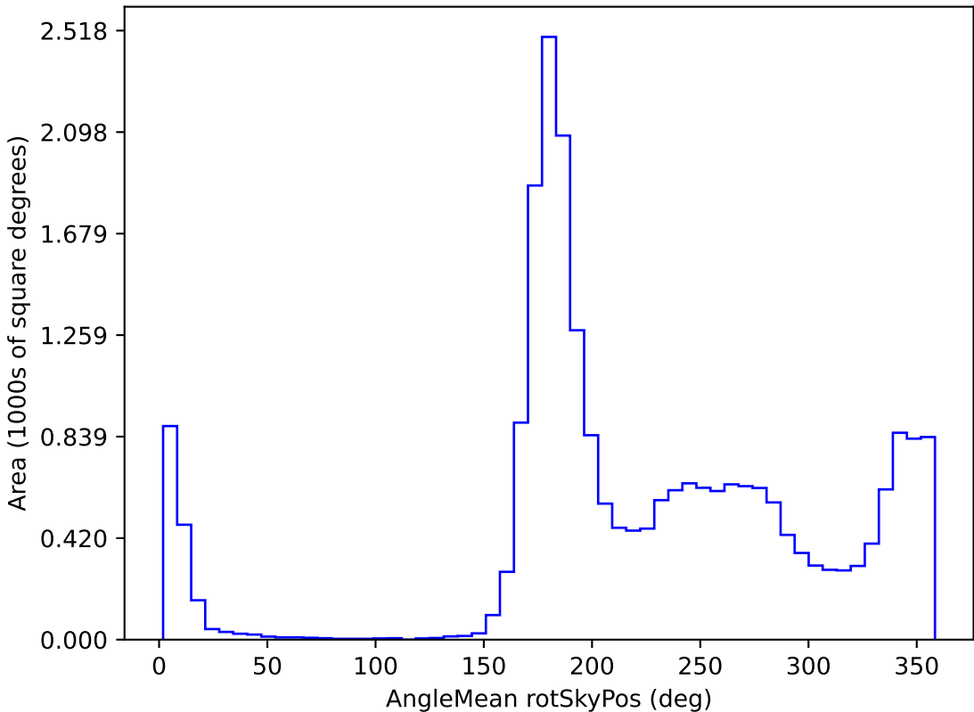
ddf_loaded_half_fl1_v3.4_10yrs All sky y band: AngleMean rotSkyPos
