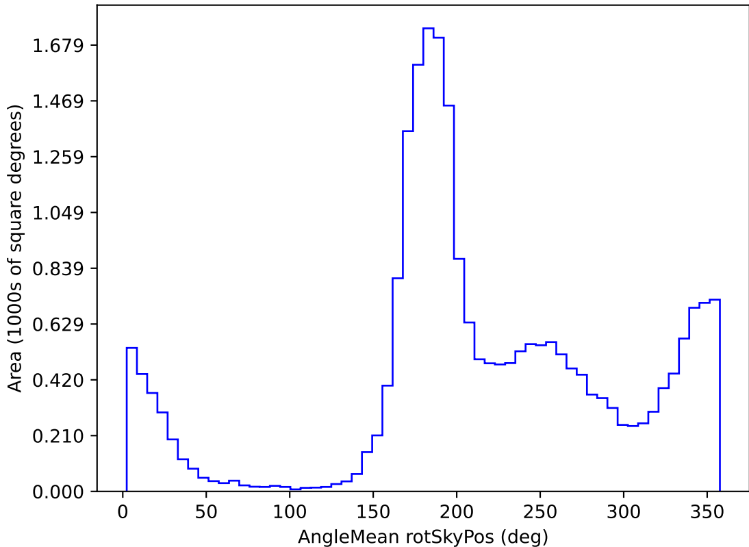
ddf_loaded_half_fl1_v3.4_10yrs All sky u band: AngleMean rotSkyPos
