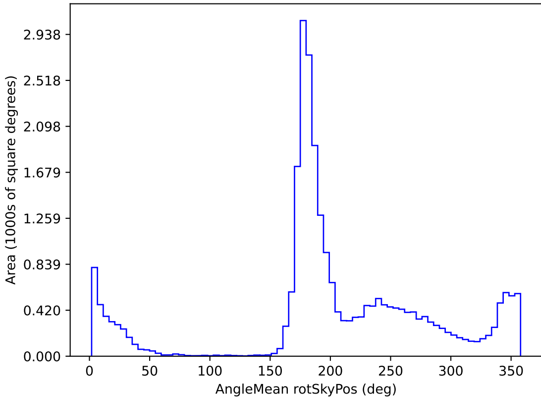
ddf_loaded_half_fl1_v3.4_10yrs All sky all bands: AngleMean rotSkyPos
