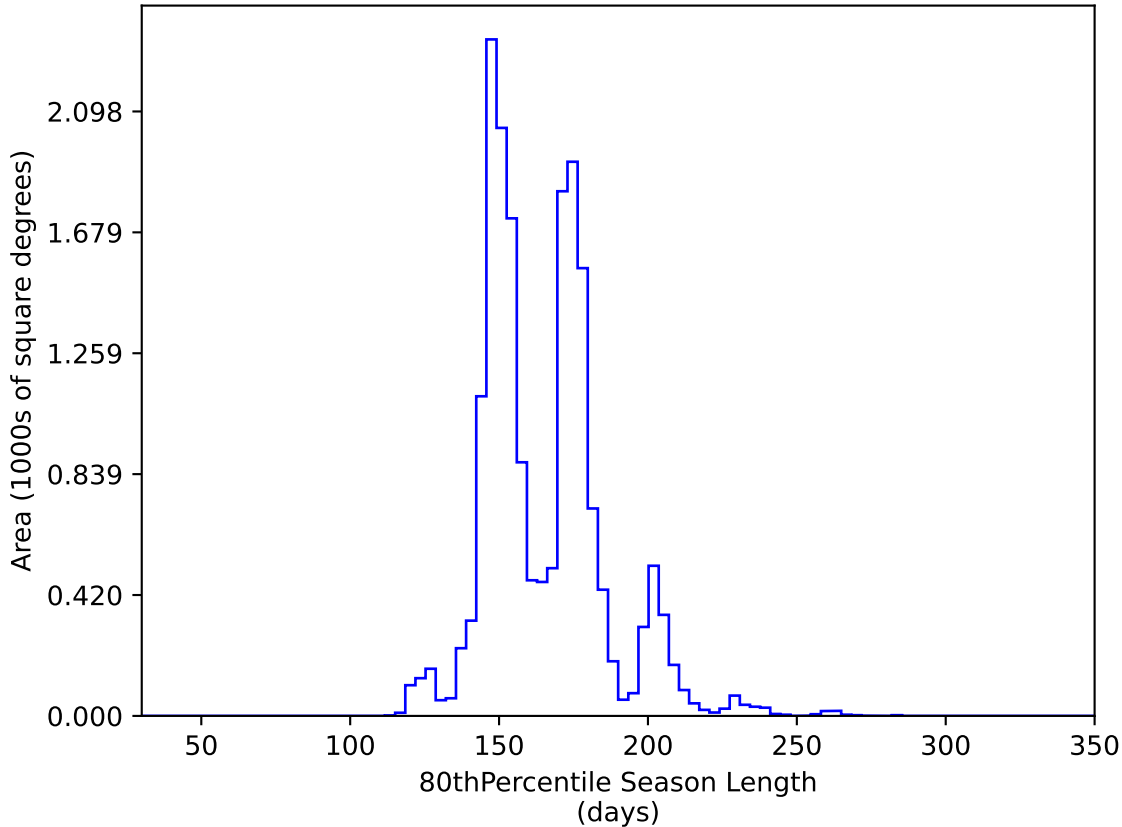
ddf_loaded_half_fl1_v3.4_10yrs WFD y band: 80thPercentile Season Length
