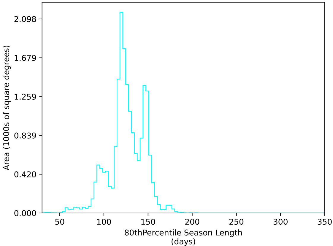
ddf_loaded_half_fl1_v3.4_10yrs WFD u band: 80thPercentile Season Length
