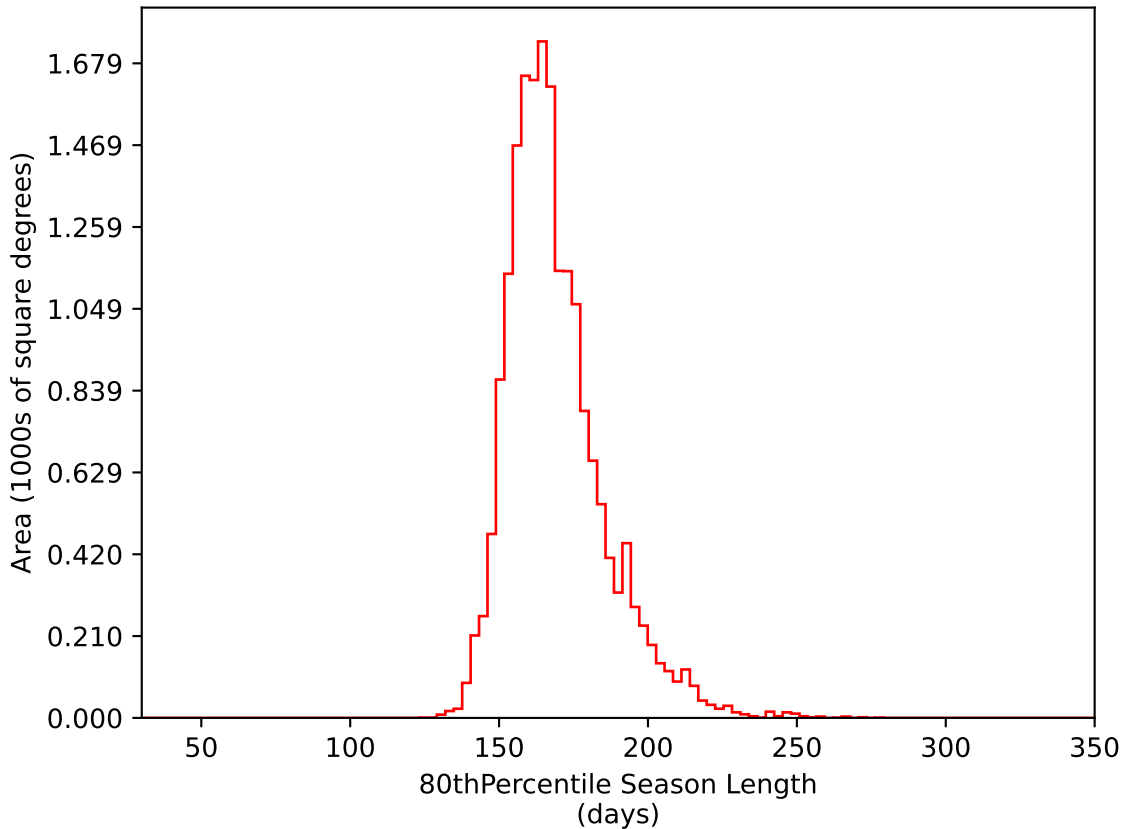
ddf_loaded_half_fl1_v3.4_10yrs WFD i band: 80thPercentile Season Length
