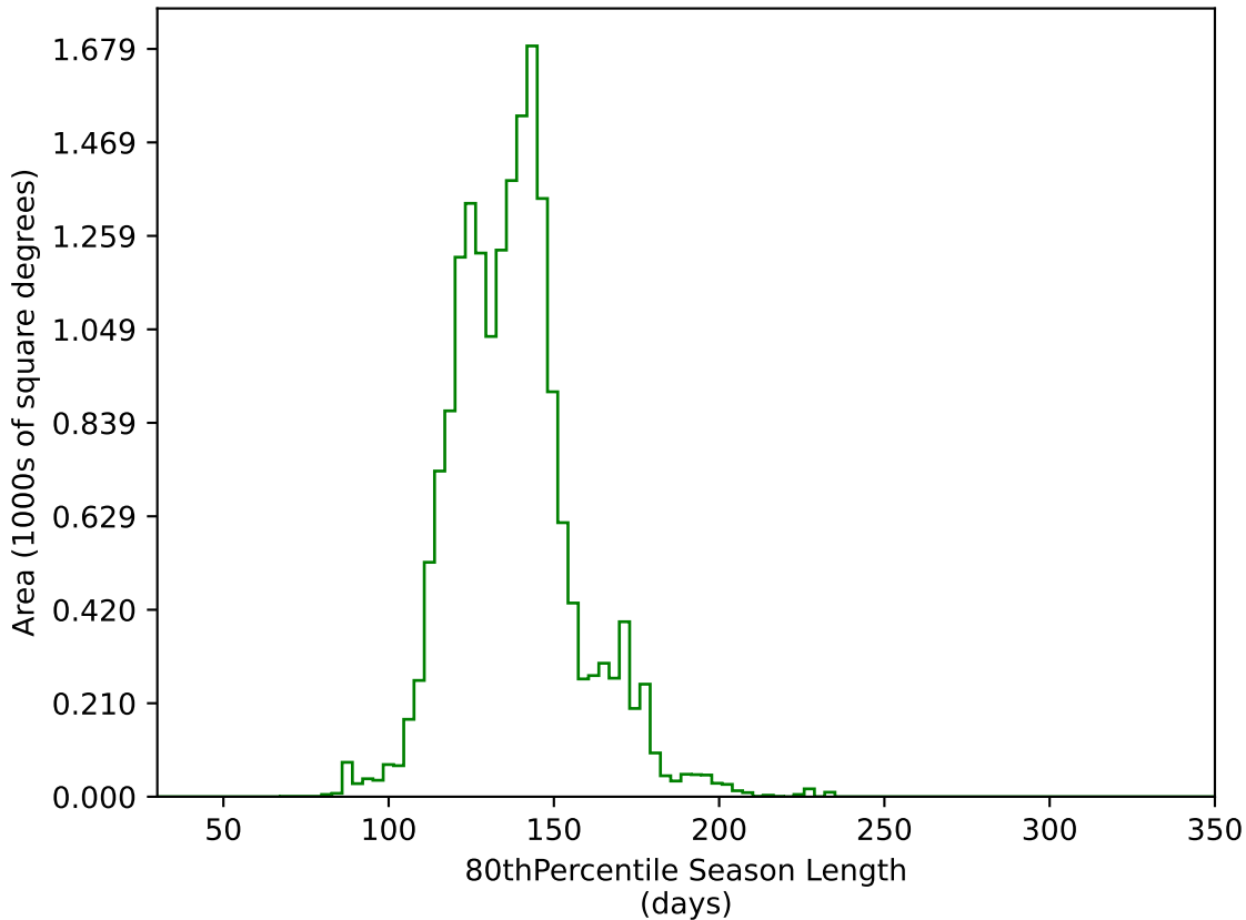
ddf_loaded_half_fl1_v3.4_10yrs WFD g band: 80thPercentile Season Length
