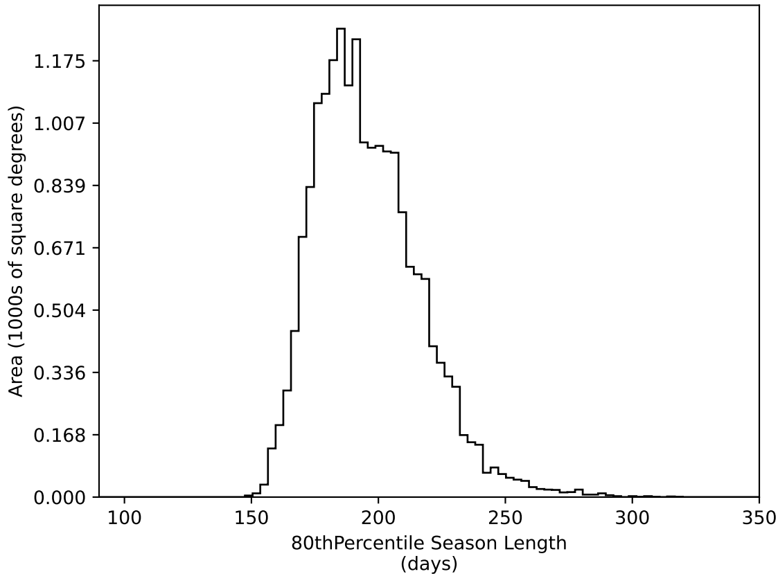
ddf_loaded_half_fl1_v3.4_10yrs WFD all bands: 80thPercentile Season Length
