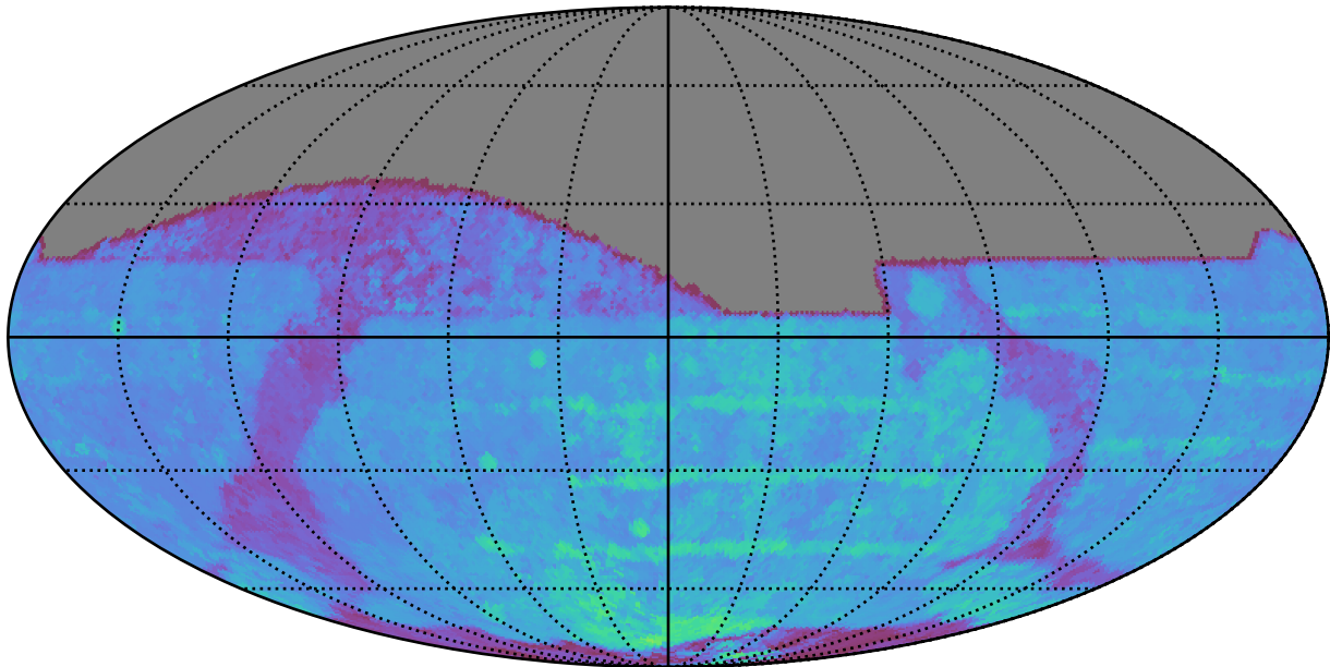
ddf_loaded_half_fl1_v3.4_10yrs All sky z band: 80thPercentile Season Length
