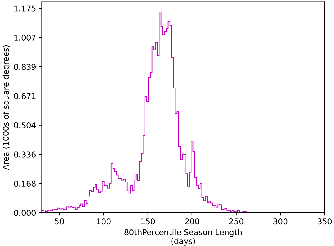
ddf_loaded_half_fl1_v3.4_10yrs All sky z band: 80thPercentile Season Length
