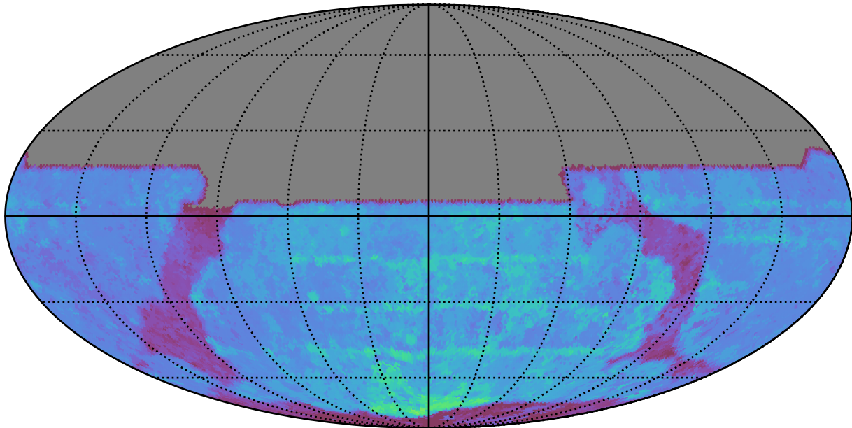
ddf_loaded_half_fl1_v3.4_10yrs All sky y band: 80thPercentile Season Length
