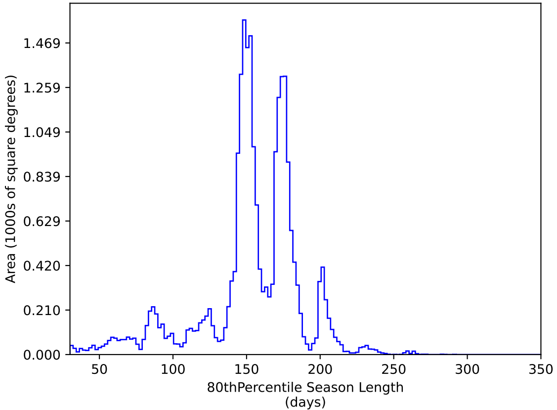
ddf_loaded_half_fl1_v3.4_10yrs All sky y band: 80thPercentile Season Length
