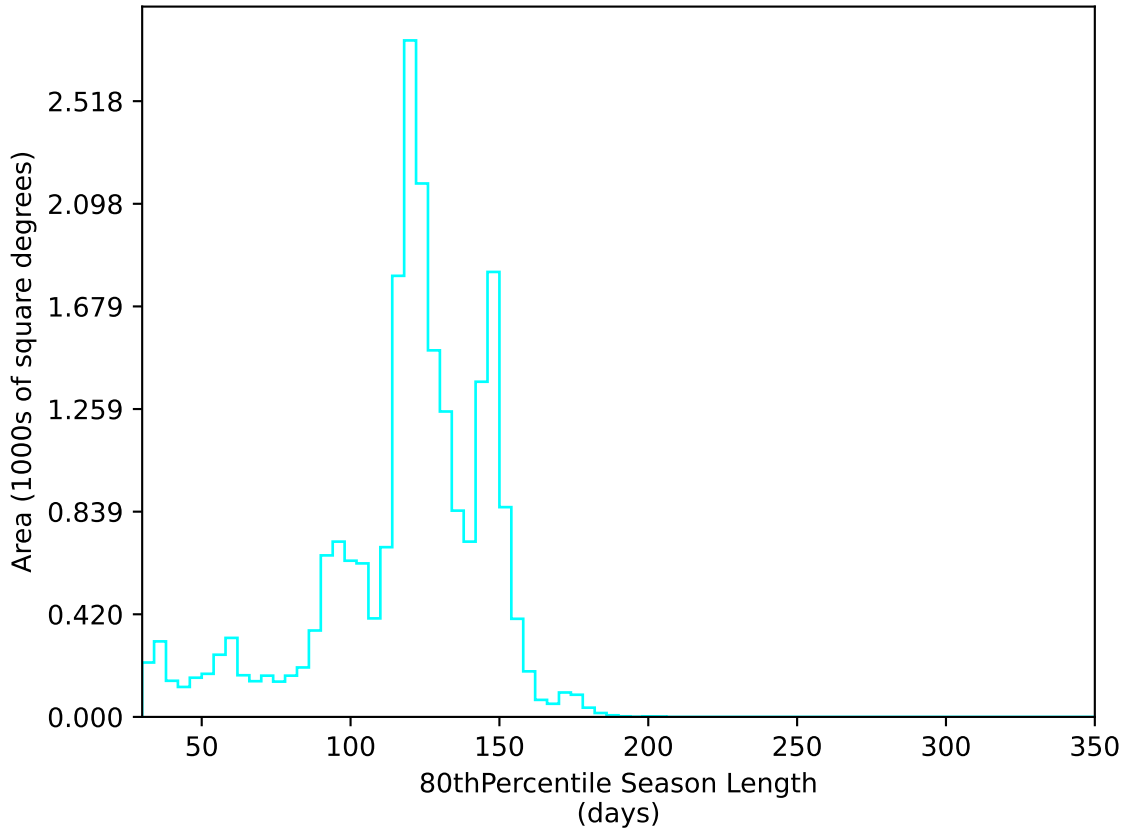
ddf_loaded_half_fl1_v3.4_10yrs All sky u band: 80thPercentile Season Length
