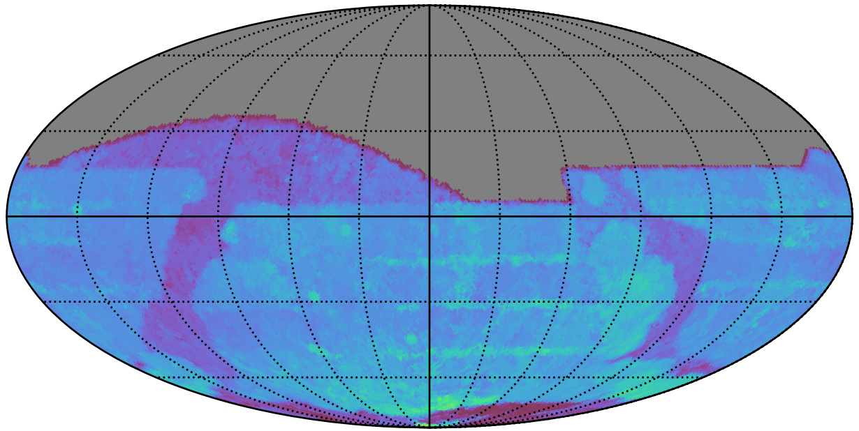
ddf_loaded_half_fl1_v3.4_10yrs All sky r band: 80thPercentile Season Length
