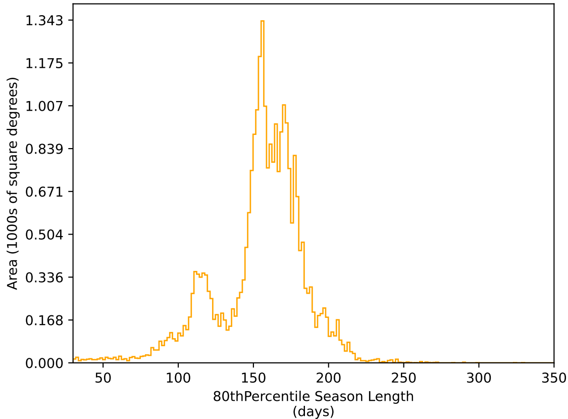
ddf_loaded_half_fl1_v3.4_10yrs All sky r band: 80thPercentile Season Length
