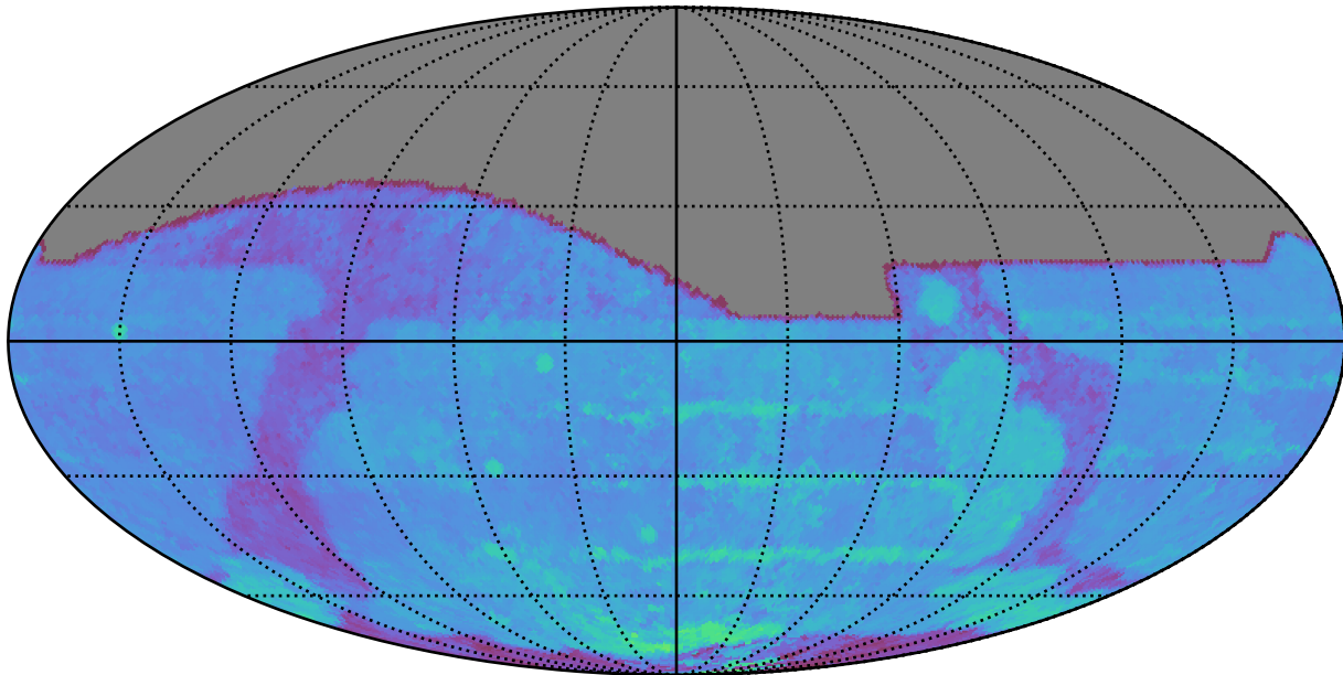
ddf_loaded_half_fl1_v3.4_10yrs All sky i band: 80thPercentile Season Length
