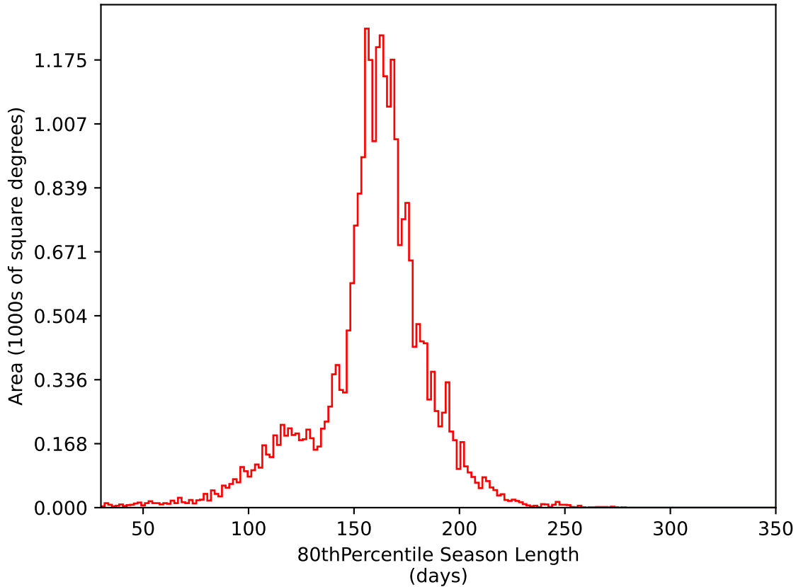
ddf_loaded_half_fl1_v3.4_10yrs All sky i band: 80thPercentile Season Length
