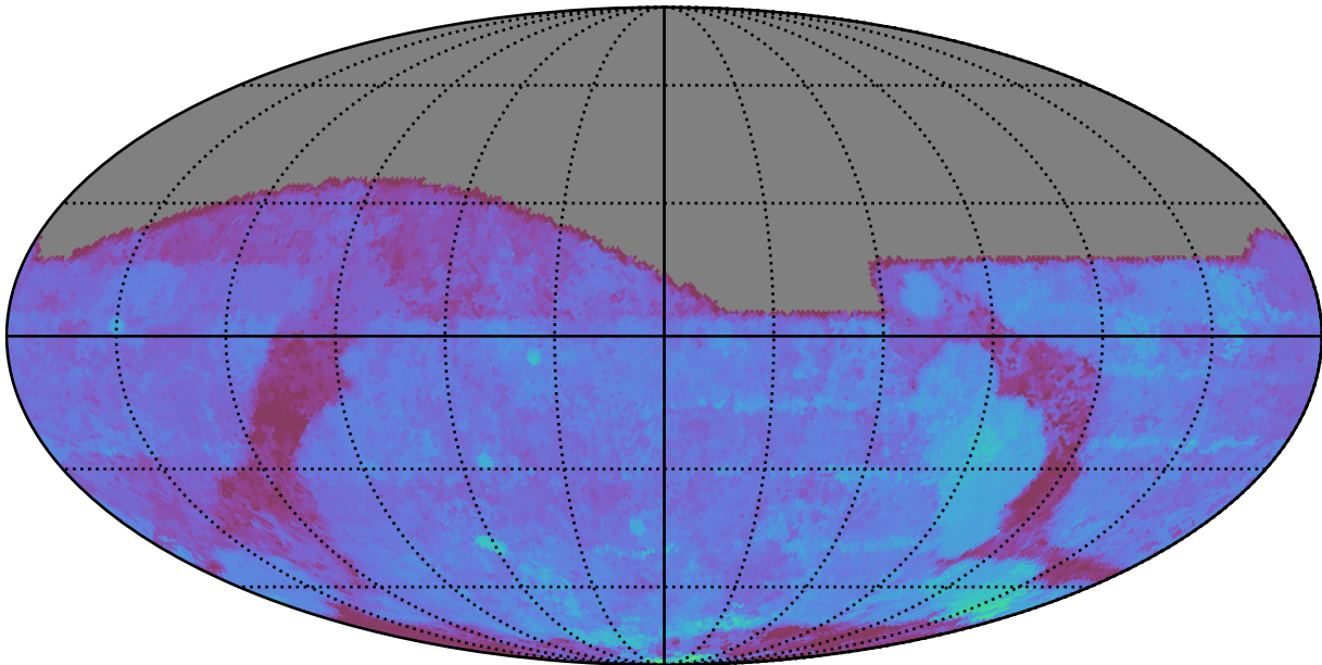
ddf_loaded_half_fl1_v3.4_10yrs All sky g band: 80thPercentile Season Length
