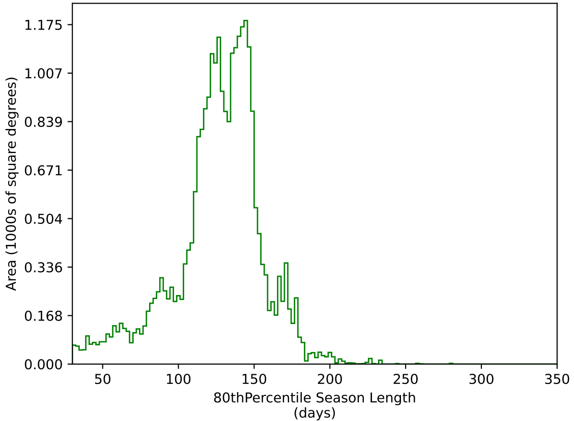
ddf_loaded_half_fl1_v3.4_10yrs All sky g band: 80thPercentile Season Length
