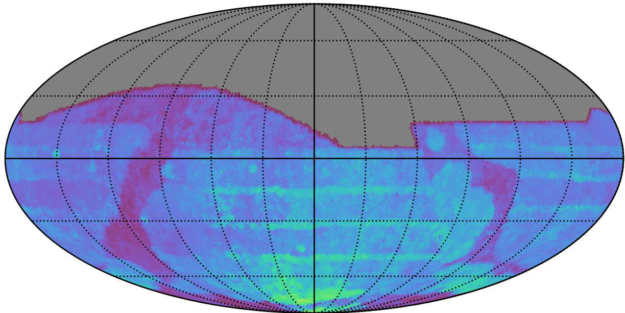
ddf_loaded_half_fl1_v3.4_10yrs All sky all bands: 80thPercentile Season Length
