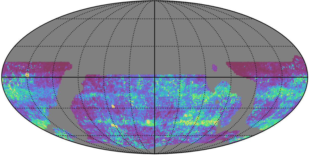
ddf_loaded_half_fl1_v3.4_10yrs WFD zy bands: 75th Percentile Intranight Timespan
