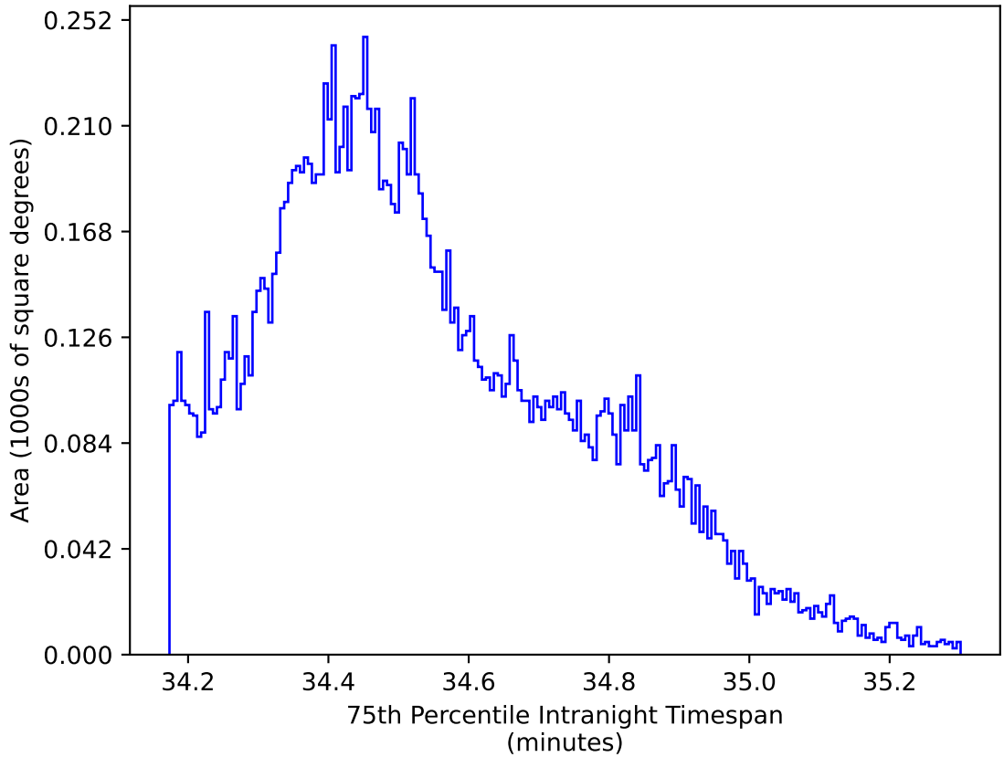
ddf_loaded_half_fl1_v3.4_10yrs WFD zy bands: 75th Percentile Intranight Timespan
