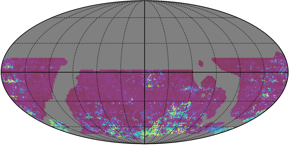
ddf_loaded_half_fl1_v3.4_10yrs WFD z band: 75th Percentile Intranight Timespan
