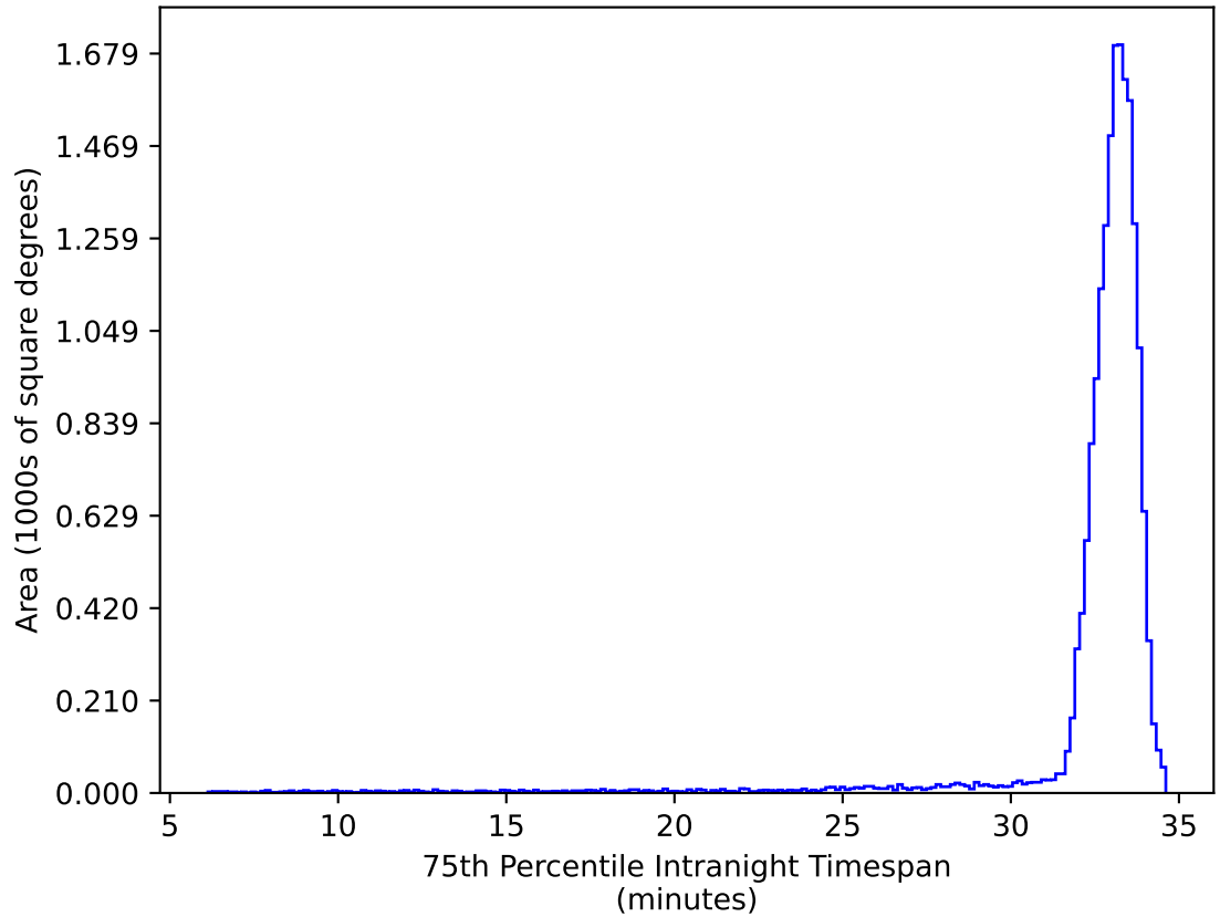
ddf_loaded_half_fl1_v3.4_10yrs WFD ug bands: 75th Percentile Intranight Timespan
