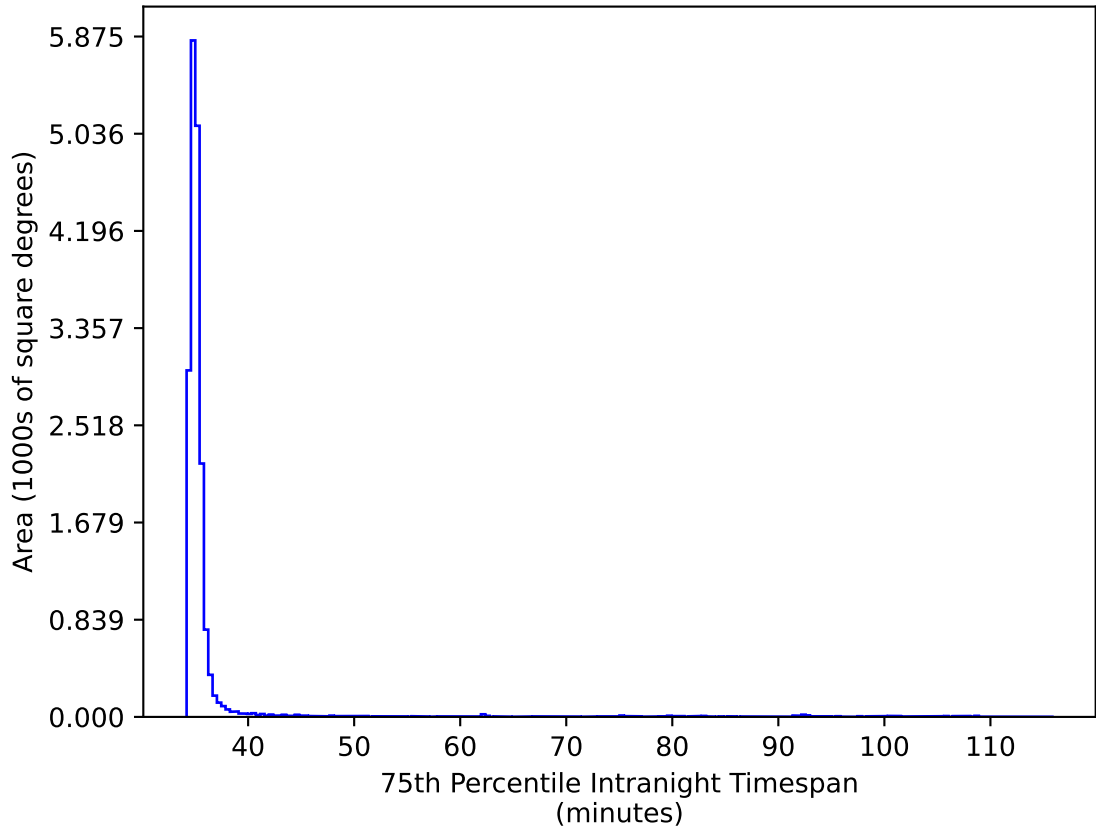
ddf_loaded_half_fl1_v3.4_10yrs WFD ri bands: 75th Percentile Intranight Timespan
