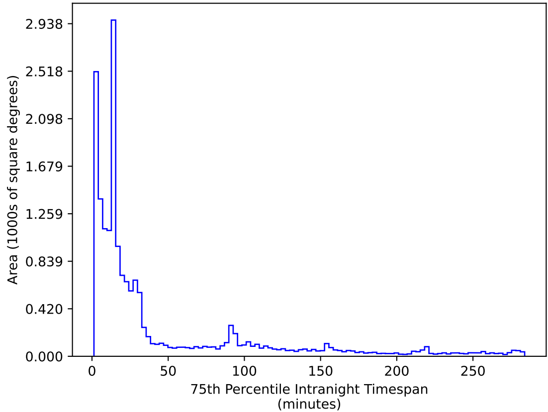
ddf_loaded_half_fl1_v3.4_10yrs WFD r band: 75th Percentile Intranight Timespan
