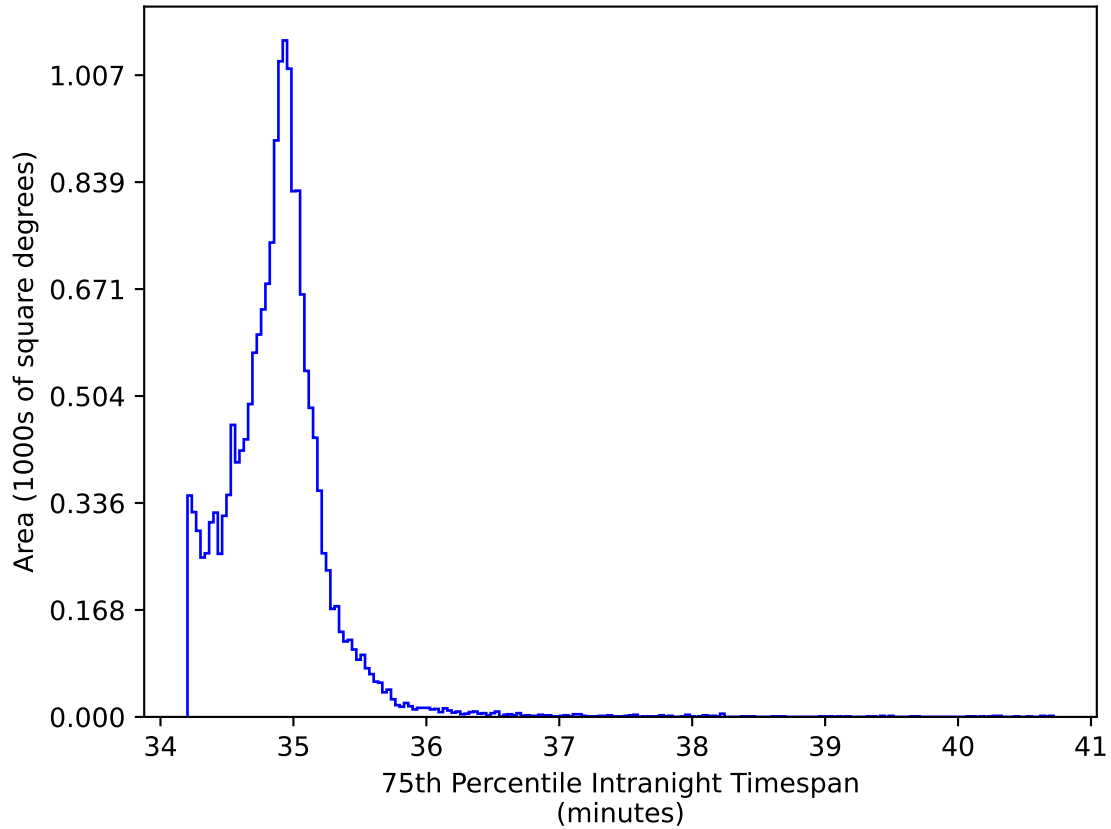
ddf_loaded_half_fl1_v3.4_10yrs WFD iz bands: 75th Percentile Intranight Timespan
