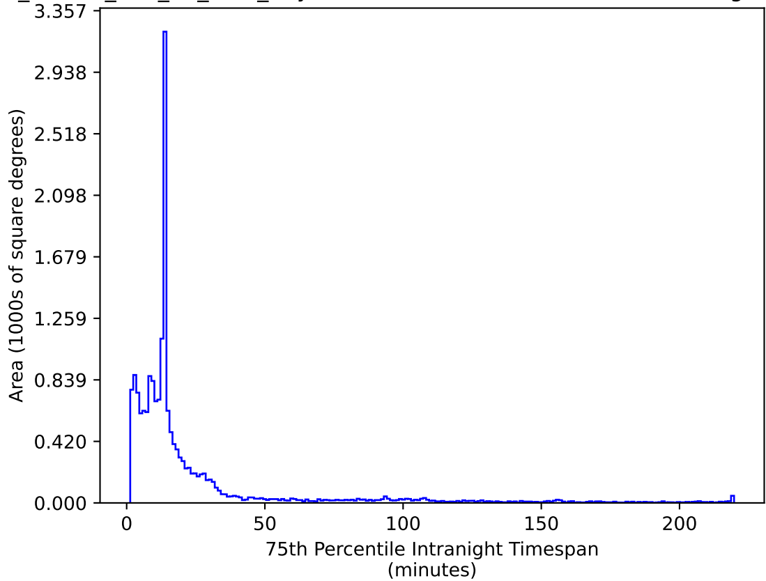
ddf_loaded_half_fl1_v3.4_10yrs WFD i band: 75th Percentile Intranight Timespan
