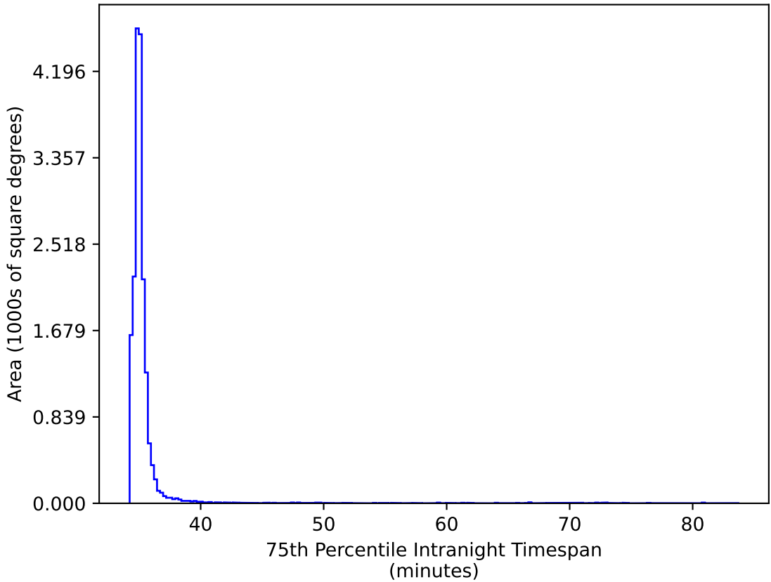
ddf_loaded_half_fl1_v3.4_10yrs WFD gr bands: 75th Percentile Intranight Timespan
