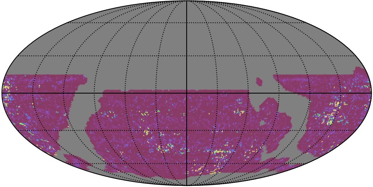
ddf_loaded_half_fl1_v3.4_10yrs WFD g band: 75th Percentile Intranight Timespan
