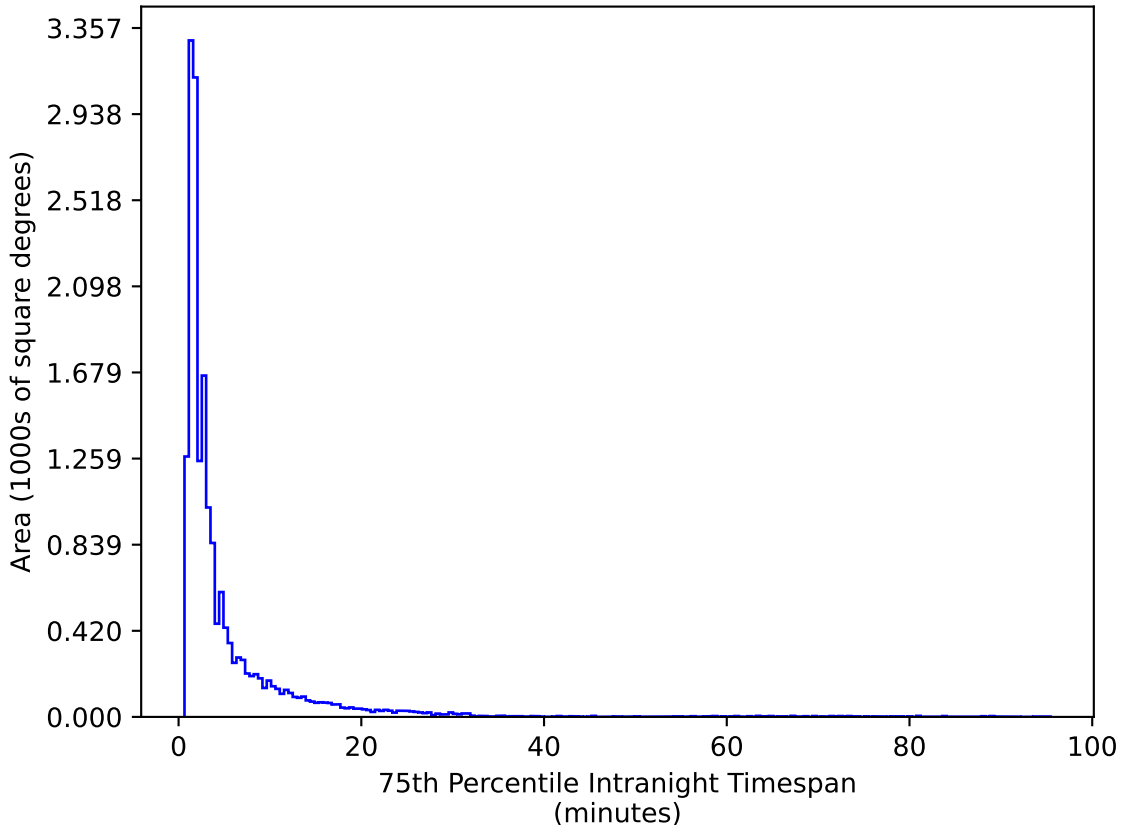
ddf_loaded_half_fl1_v3.4_10yrs WFD g band: 75th Percentile Intranight Timespan
