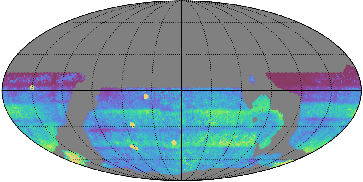
ddf_loaded_half_fl1_v3.4_10yrs WFD all bands: 75th Percentile Intranight Timespan
