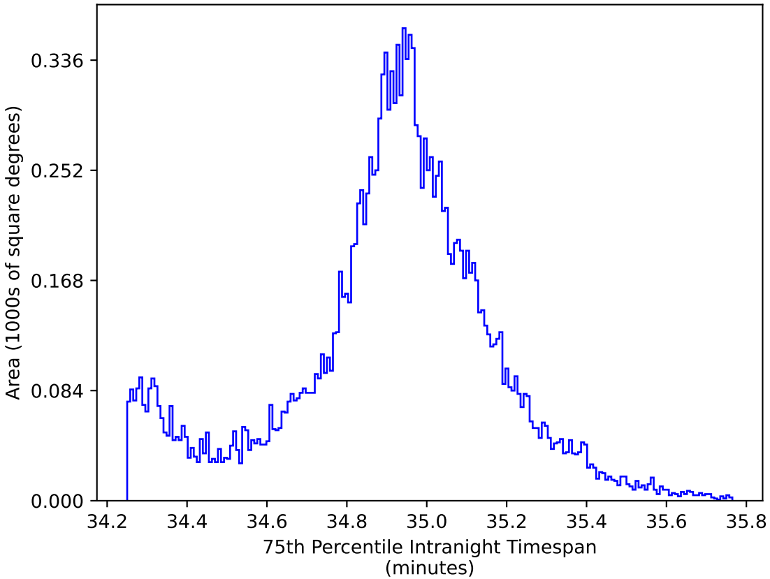
ddf_loaded_half_fl1_v3.4_10yrs WFD: 75th Percentile Intranight Timespan
