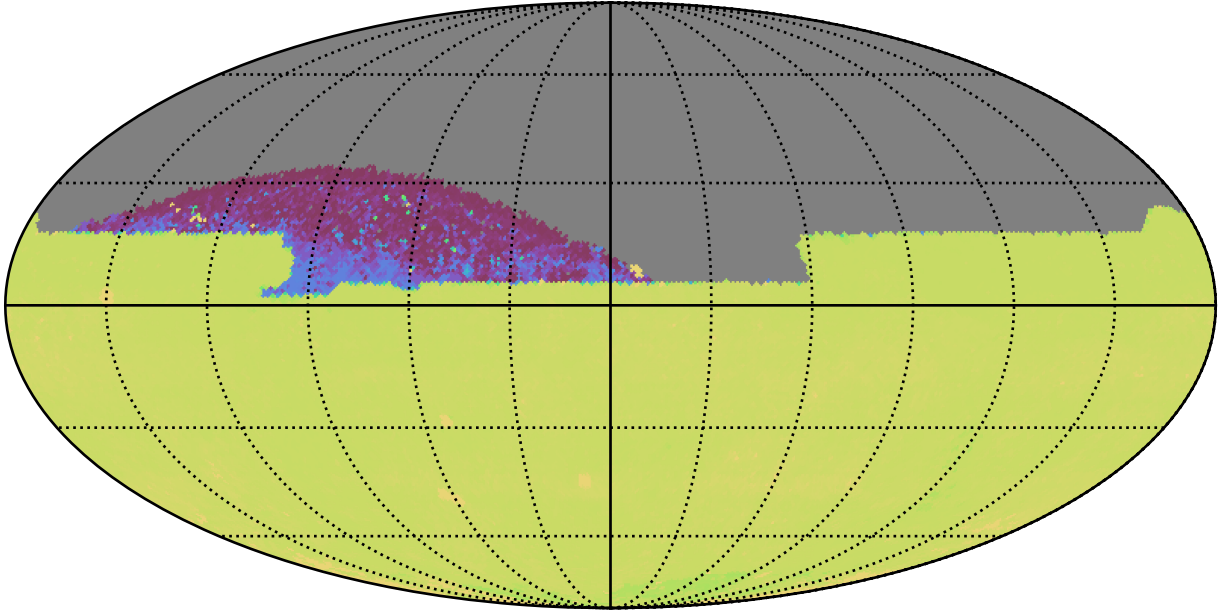
ddf_loaded_half_fl1_v3.4_10yrs All sky zy bands: 75th Percentile Intranight Timespan
