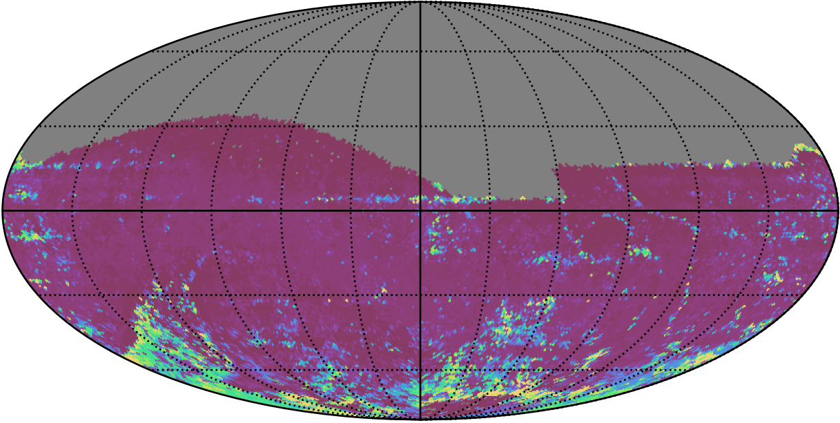
ddf_loaded_half_fl1_v3.4_10yrs All sky z band: 75th Percentile Intranight Timespan
