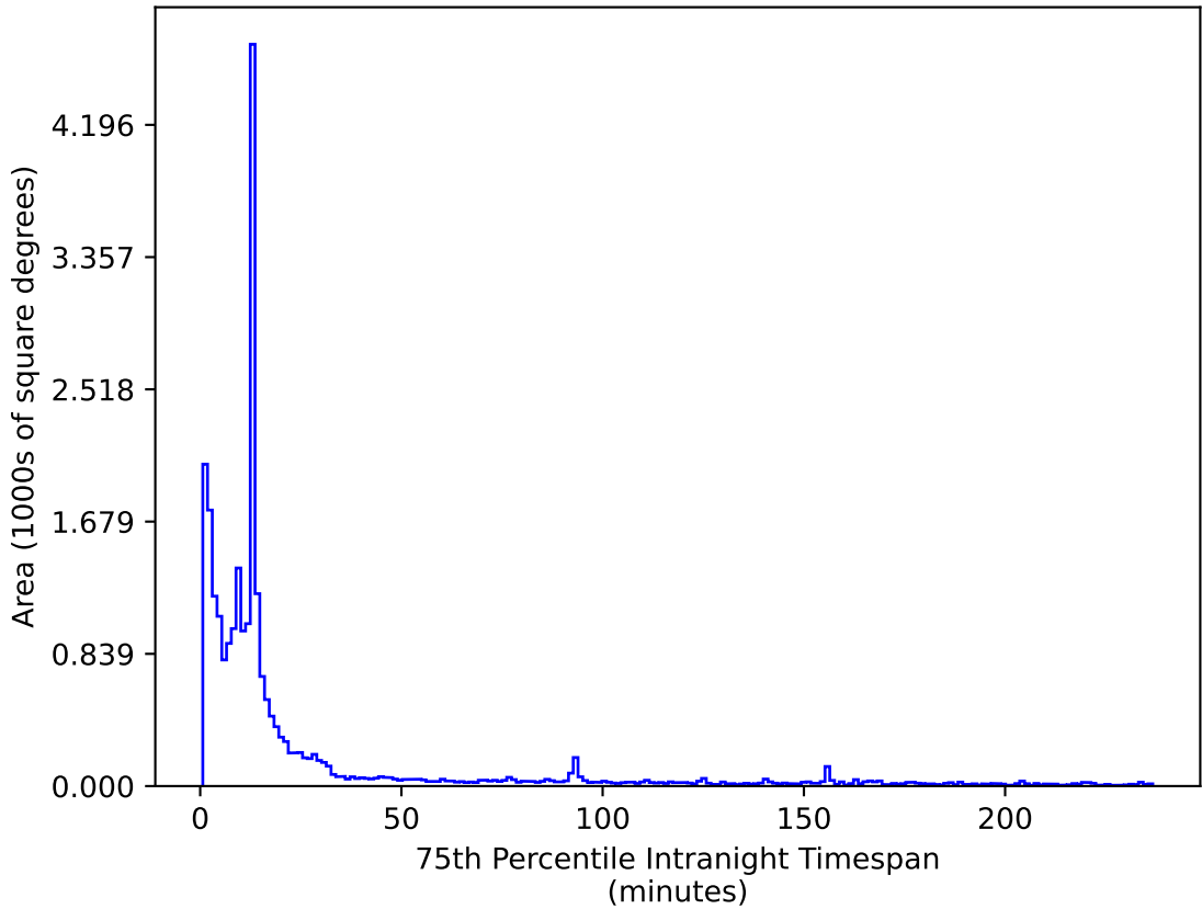
ddf_loaded_half_fl1_v3.4_10yrs All sky z band: 75th Percentile Intranight Timespan
