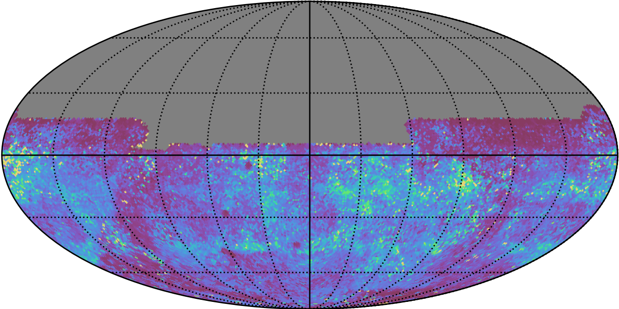
ddf_loaded_half_fl1_v3.4_10yrs All sky y band: 75th Percentile Intranight Timespan
