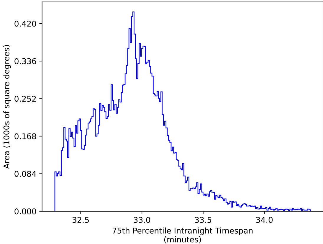
ddf_loaded_half_fl1_v3.4_10yrs All sky y band: 75th Percentile Intranight Timespan
