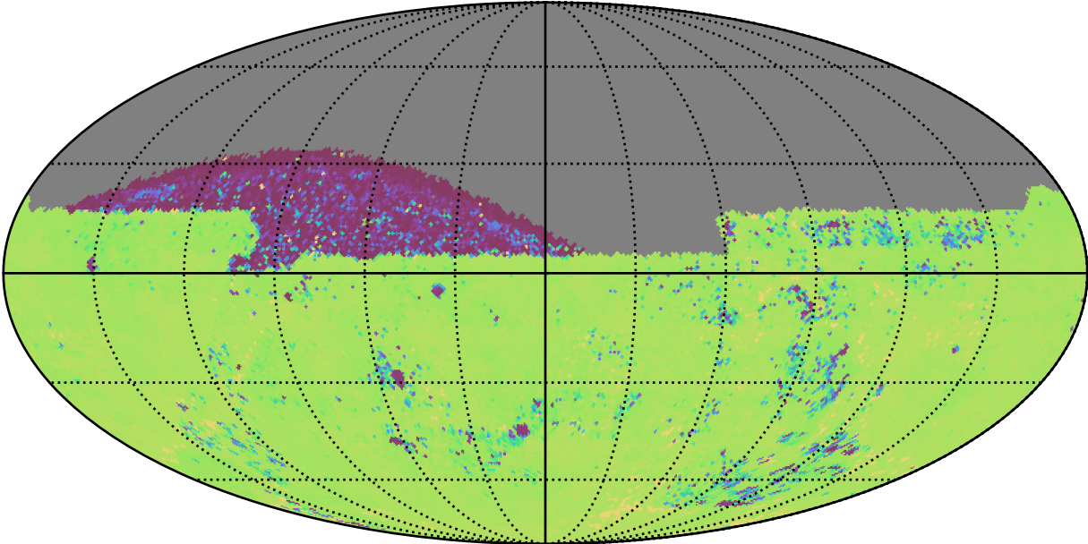
ddf_loaded_half_fl1_v3.4_10yrs All sky ug bands: 75th Percentile Intranight Timespan
