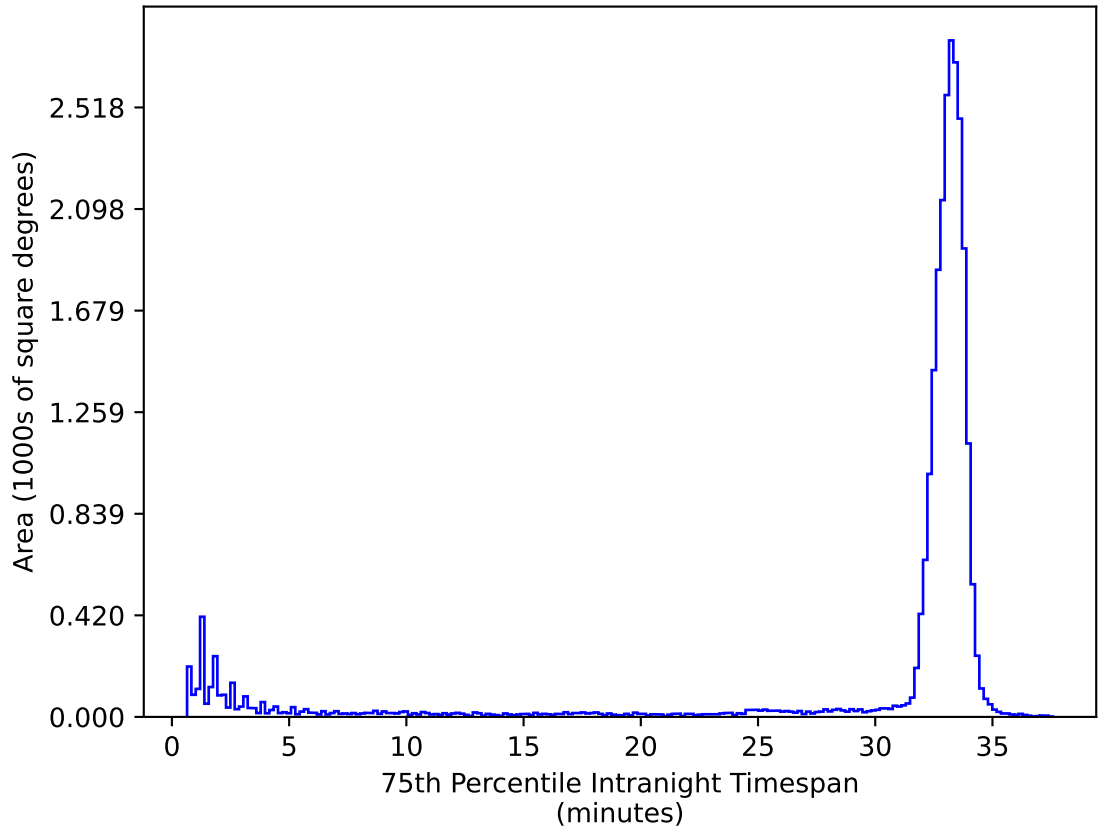
ddf_loaded_half_fl1_v3.4_10yrs All sky ug bands: 75th Percentile Intranight Timespan
