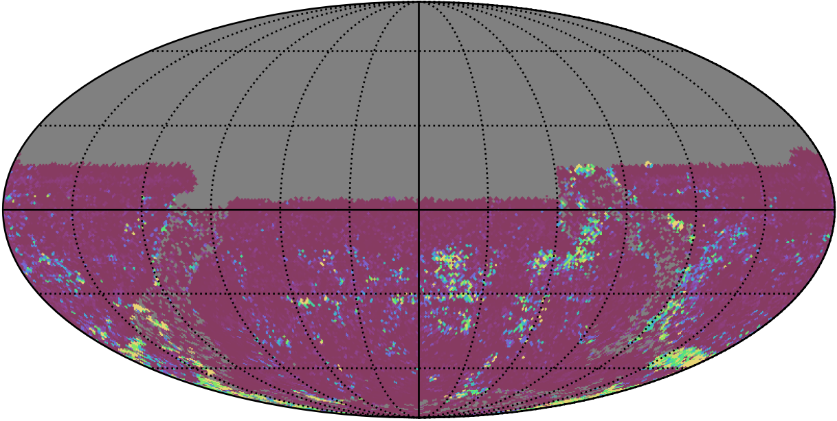
ddf_loaded_half_fl1_v3.4_10yrs All sky u band: 75th Percentile Intranight Timespan
