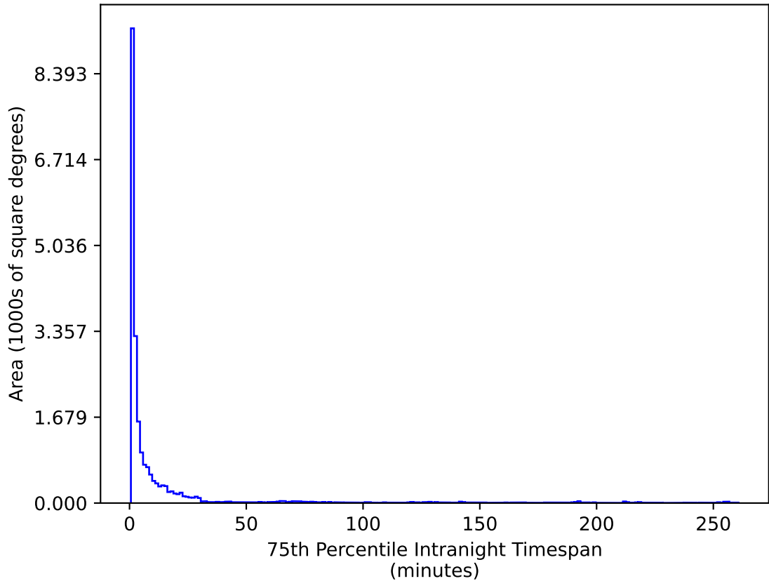
ddf_loaded_half_fl1_v3.4_10yrs All sky u band: 75th Percentile Intranight Timespan
