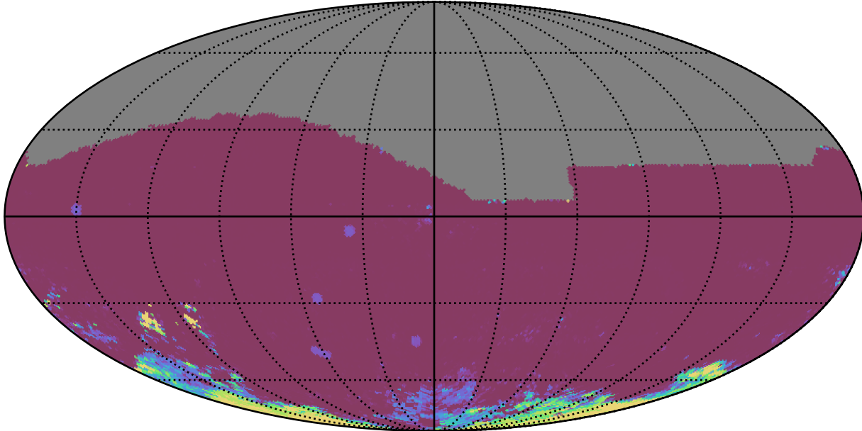
ddf_loaded_half_fl1_v3.4_10yrs All sky ri bands: 75th Percentile Intranight Timespan
