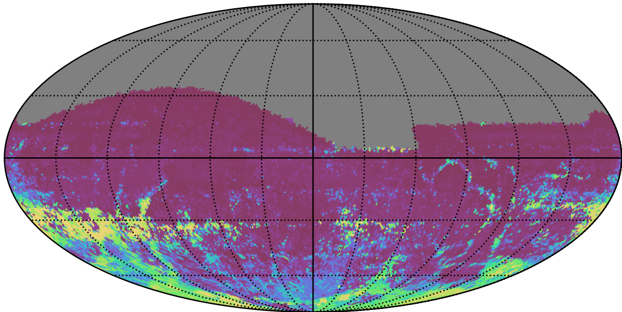
ddf_loaded_half_fl1_v3.4_10yrs All sky r band: 75th Percentile Intranight Timespan
