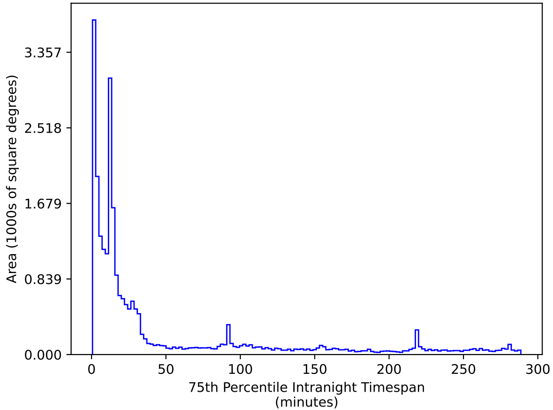
ddf_loaded_half_fl1_v3.4_10yrs All sky r band: 75th Percentile Intranight Timespan
