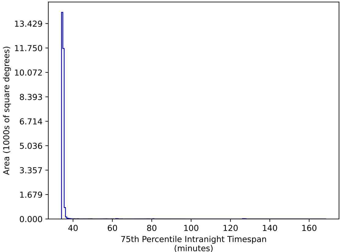
ddf_loaded_half_fl1_v3.4_10yrs All sky iz bands: 75th Percentile Intranight Timespan
